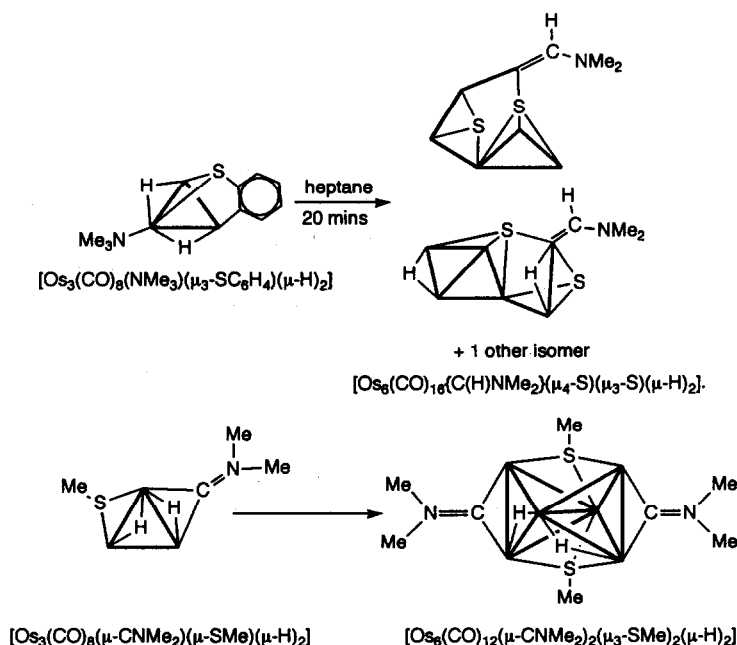
Scheme 10.
