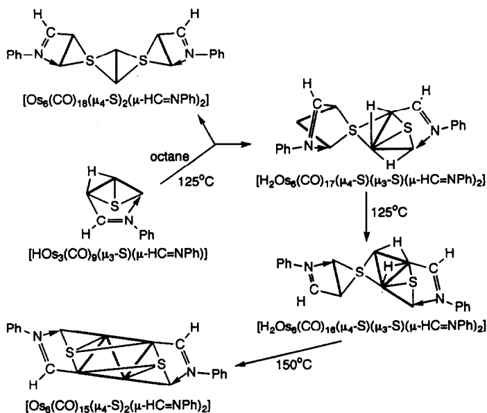
Scheme 11.
