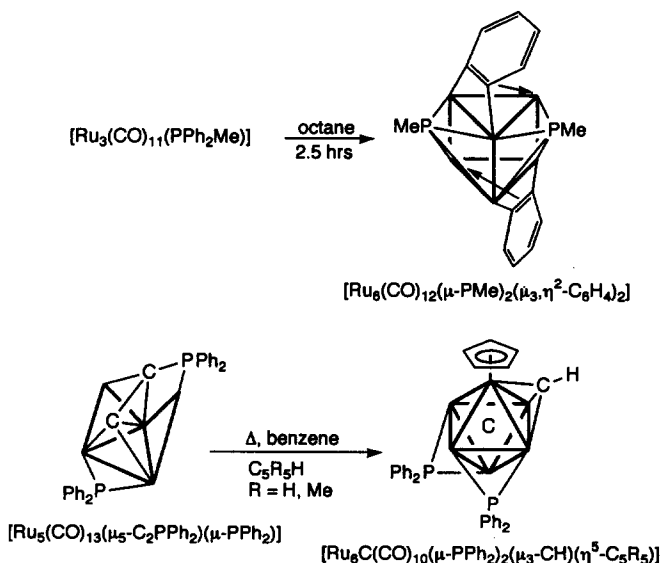
Scheme 8.
